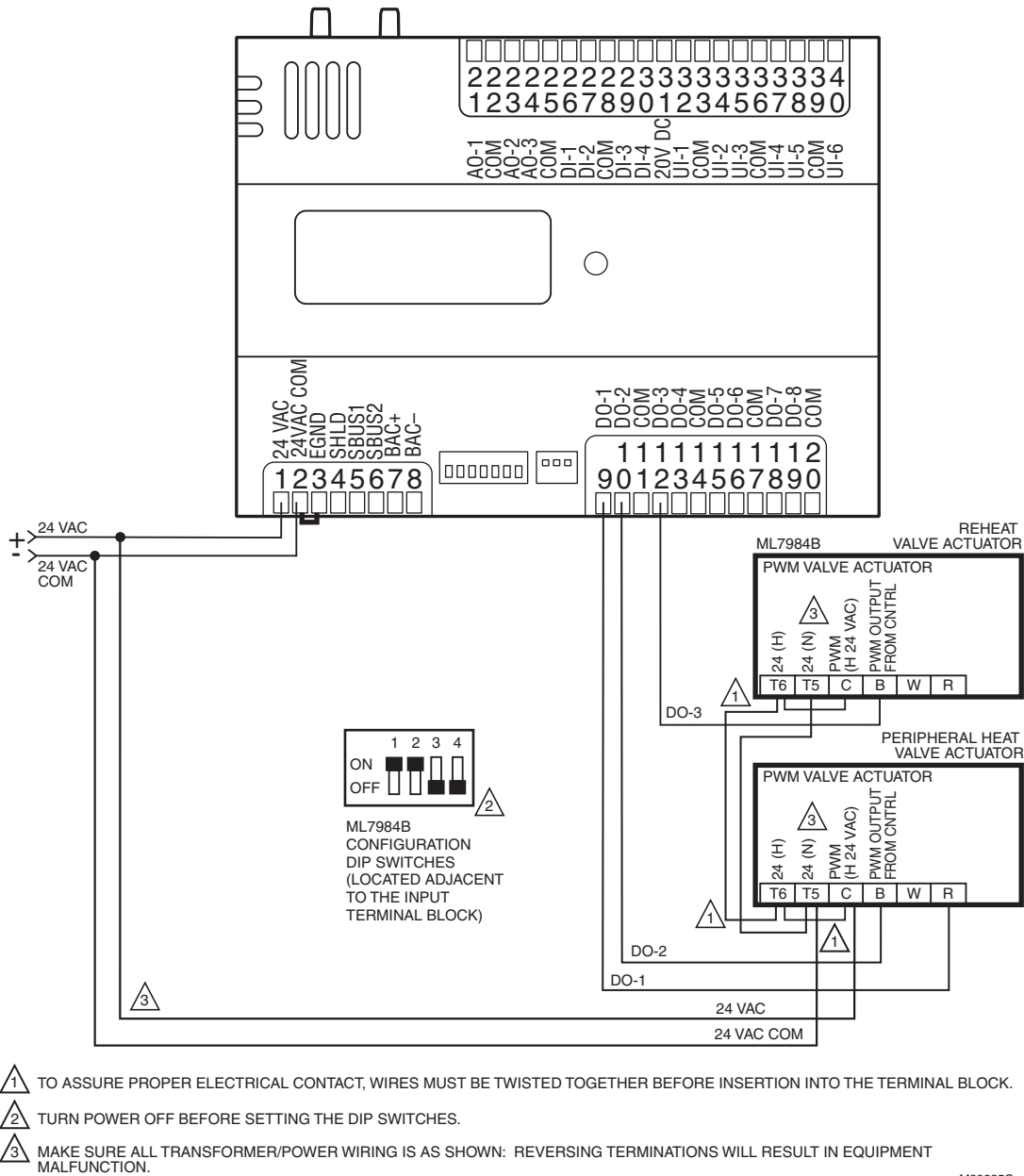
Fig. 19. Controller wiring diagram (model PUB6438S shown) for typical PWM reheat and PWM peripheral heat valve actuator. (For note 2, refer to Fig. 14.)
