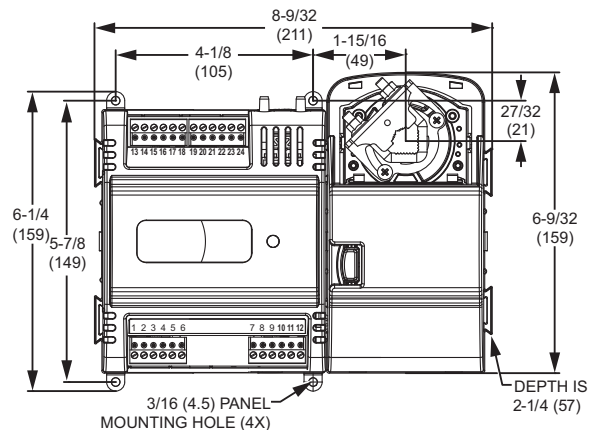
Fig. 5. Panel mounting - controller and actuator dimensions in inches (mm) for PVB0000AS and PVB4022AS only (PVB4022AS shown).
