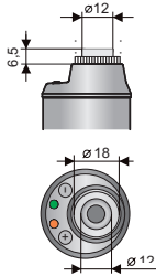
Variant "A" with short stainless steel gland
