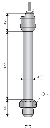
Variant "C" with connector M12
