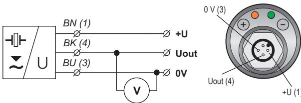
Fig. 5: Connection diagrams and interior view of connector of level meter KDLM-10 (variant - U)
