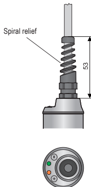
Variant "V" with plastic cable gland with spiral relief - for case of increased mechanical wear on the cable.
