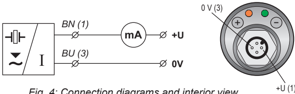
Fig. 4: Connection diagrams and interior view of connector of level meter KDLM -10 (variant - I)
